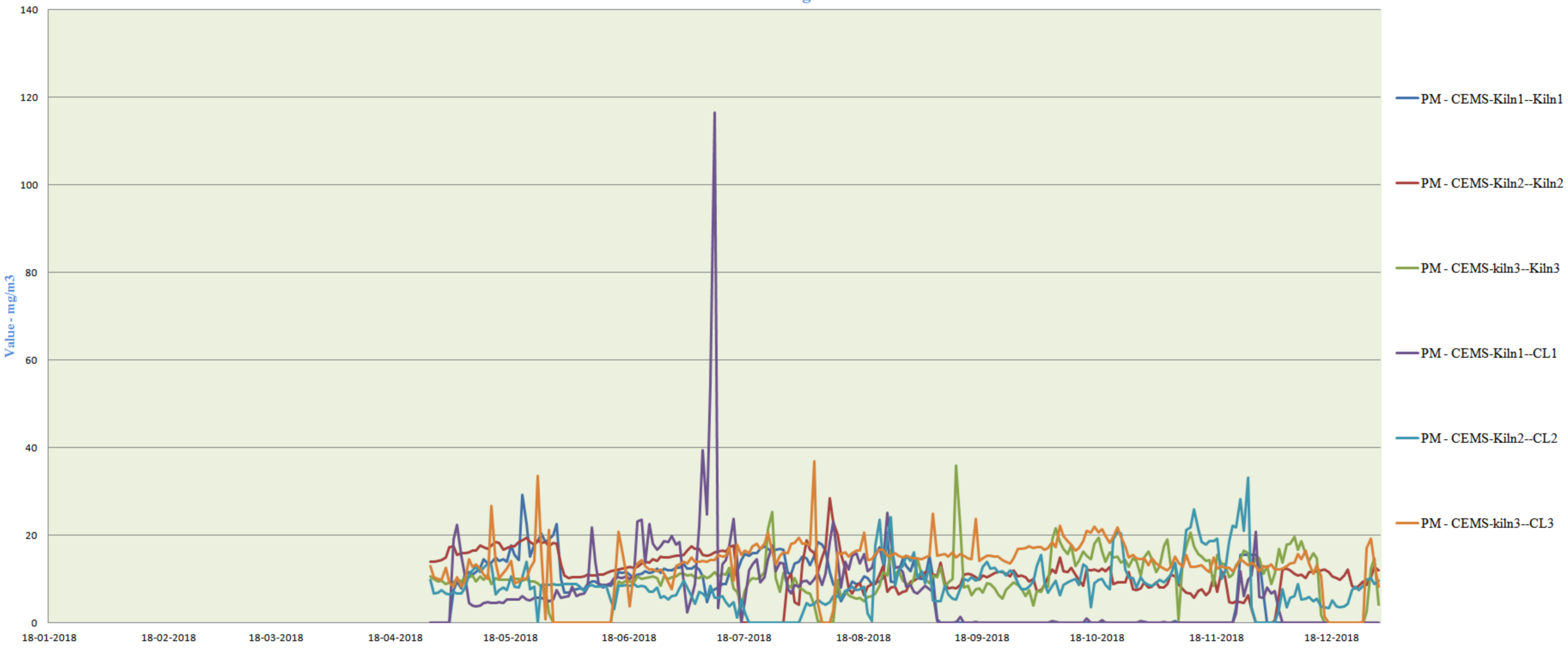
Annual Emission Trend of PM from M/s Heidelberg Cement India Ltd (Diamond Cements,Clinker Division ) - Narsingarh
